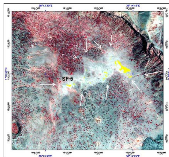
FIGURE 4: Spot image for thermal infrared for Silali caldera (GDC and BGR, 2012)
