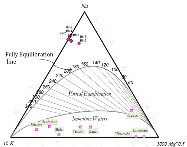
FIGURE 6: Na-K-Mg of the Logipi
