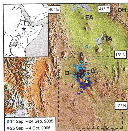
FIGURE 3: Red line shows location of dyke and red stars mark Dabbahu volcano. (From: Wright et al., 2006)
