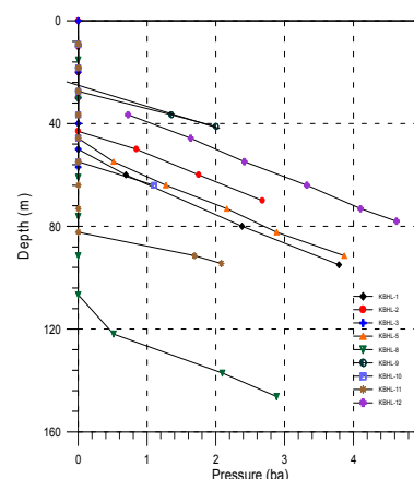
FIGURE 11: Down-hole pressure profiles
