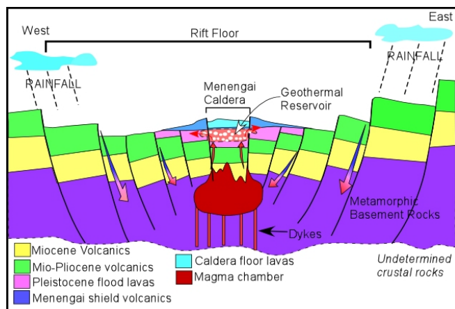
FIGURE 2: Model of a geothermal prospect in the Kenya rift
