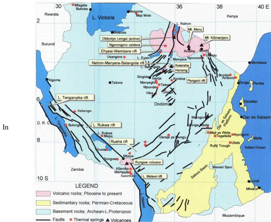
FIGURE 2: Geothermal sites in Tanzania
