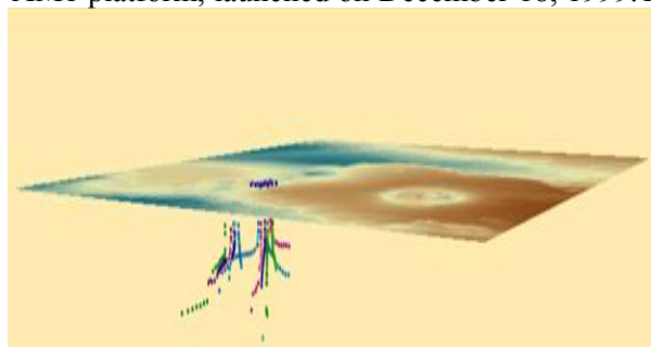
FIGURE 5a: ASTER DEM model of Olkaria geothermal field showing 3D view of geothermal directional wells.
