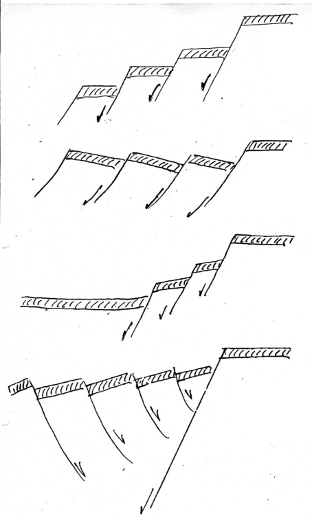
FIGURE 3: Types of normal faults
