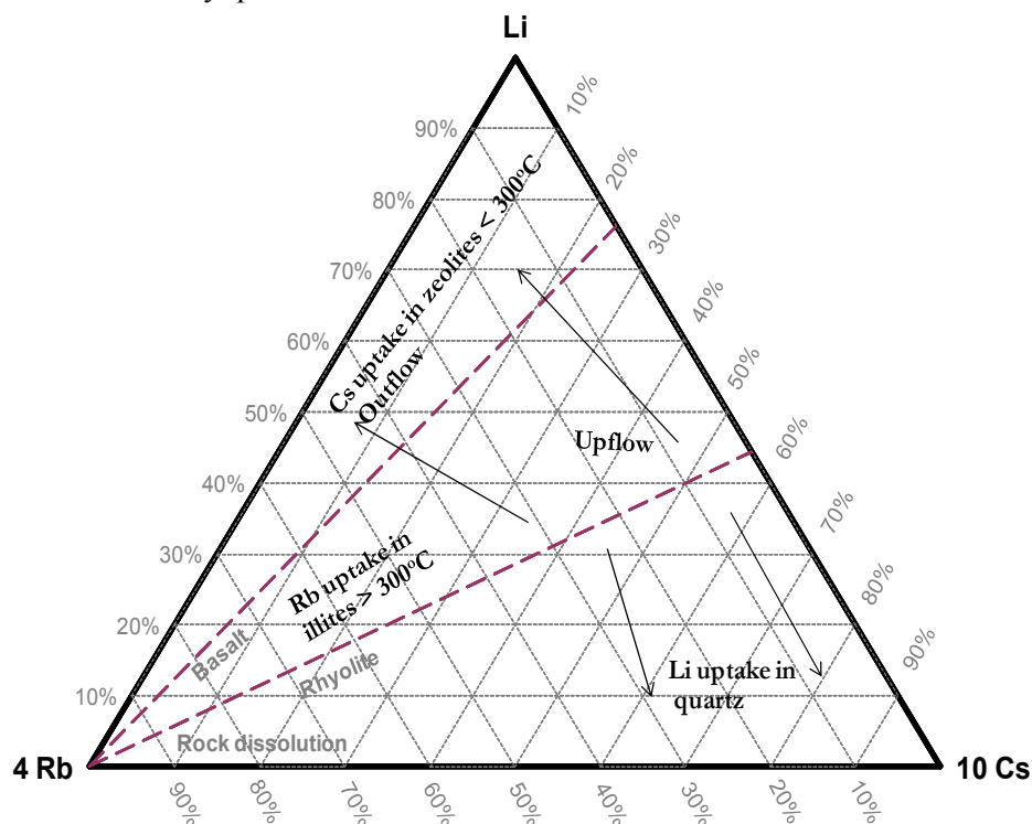
FIGURE 6: Relative Li-Rb-Cs contents
