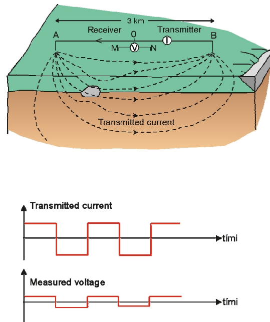
FIGURE 2: The principles behind the Schlumberger configuration and the associated current distribution in the earth
