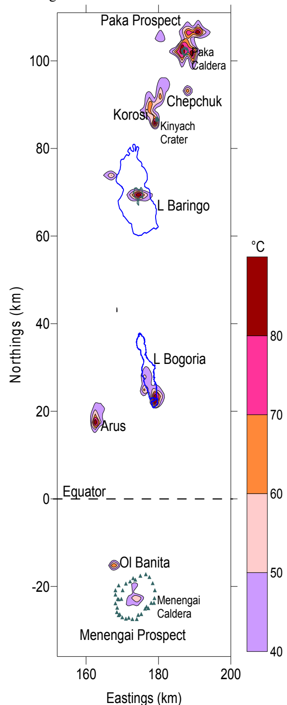
FIGURE 12: Explored prospects in the North rift
