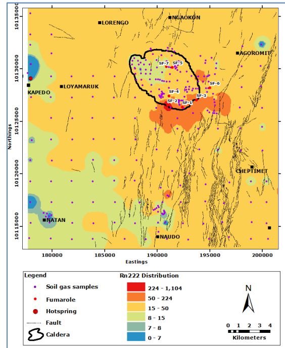
FIGURE 11: Rn-222 distribution
