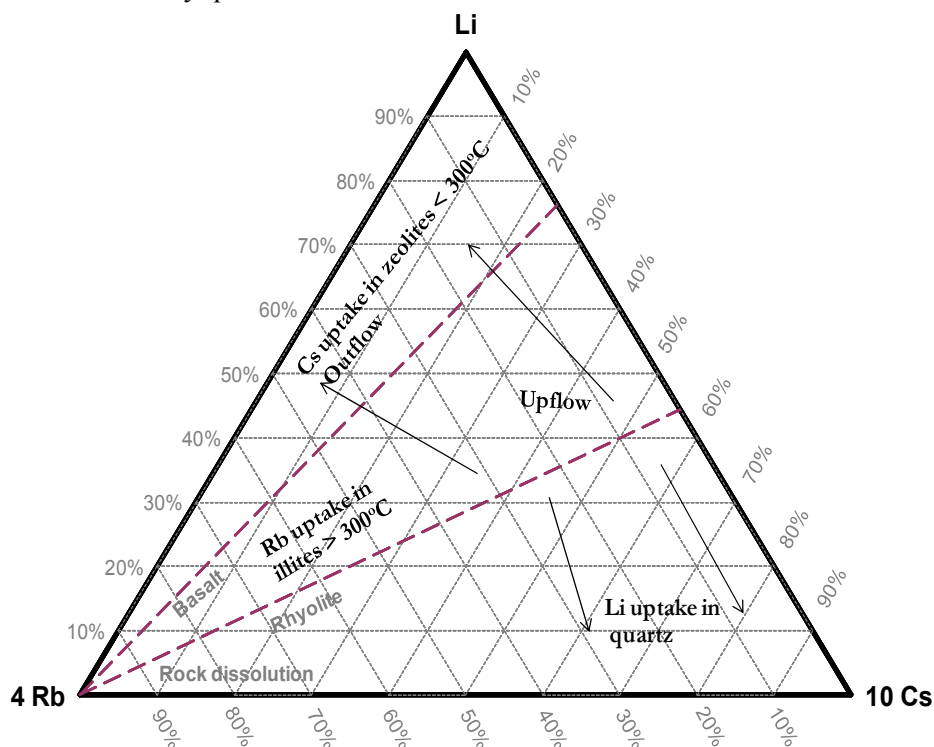
FIGURE 6: Relative Li-Rb-Cs contents
