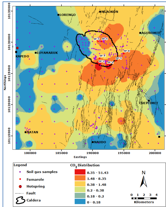
FIGURE 10: CO 2 distribution in the Silali prospect
