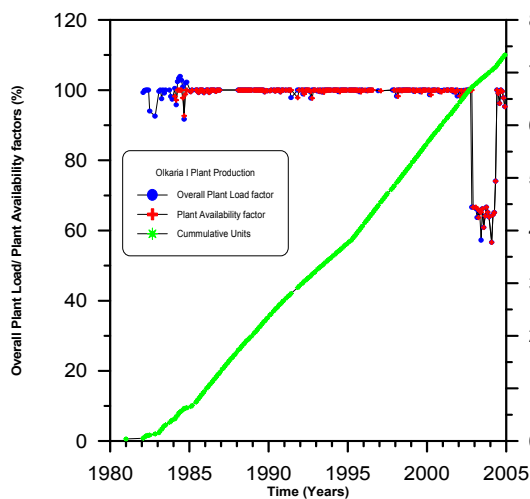
FIGURE 15: Olkaria I Plant Production
