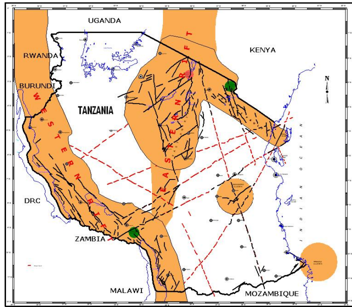
FIGURE 1: East African Rift System in Tanzania.
