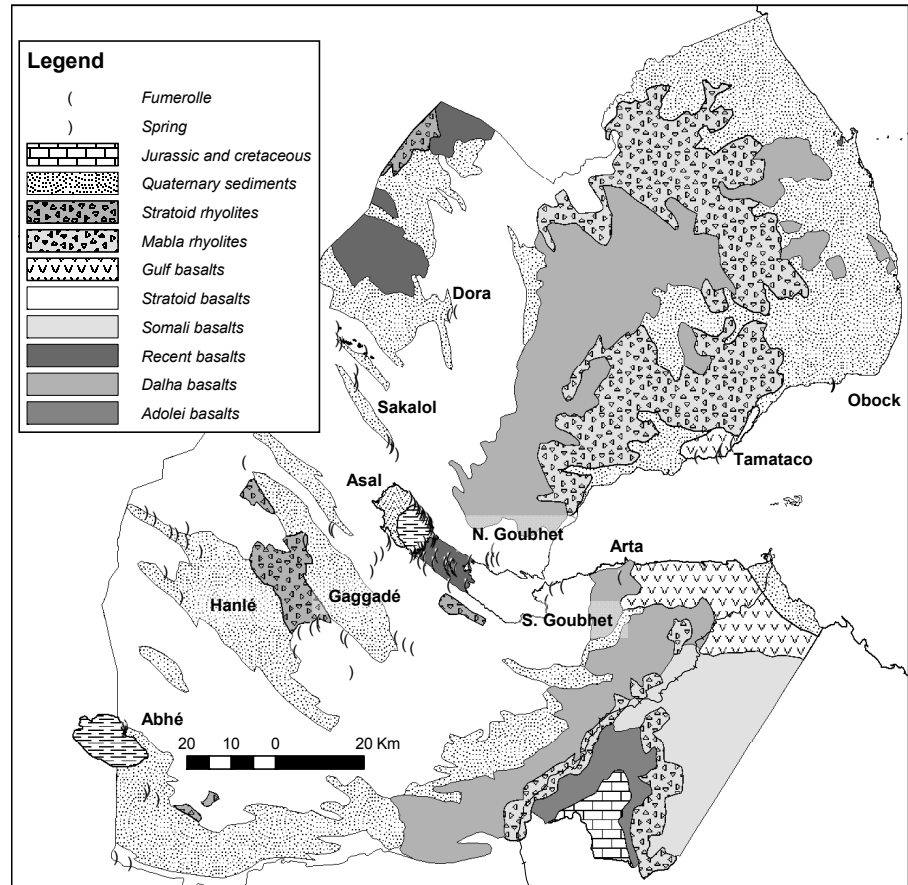
FIGURE 1: Geology and hydrothermal activity of the Republic of Djibouti
