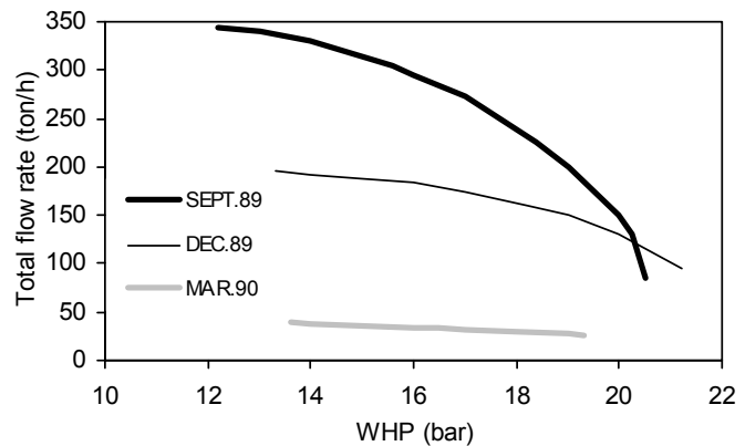
FIGURE 3: Successive output curves of the well Asal 3
