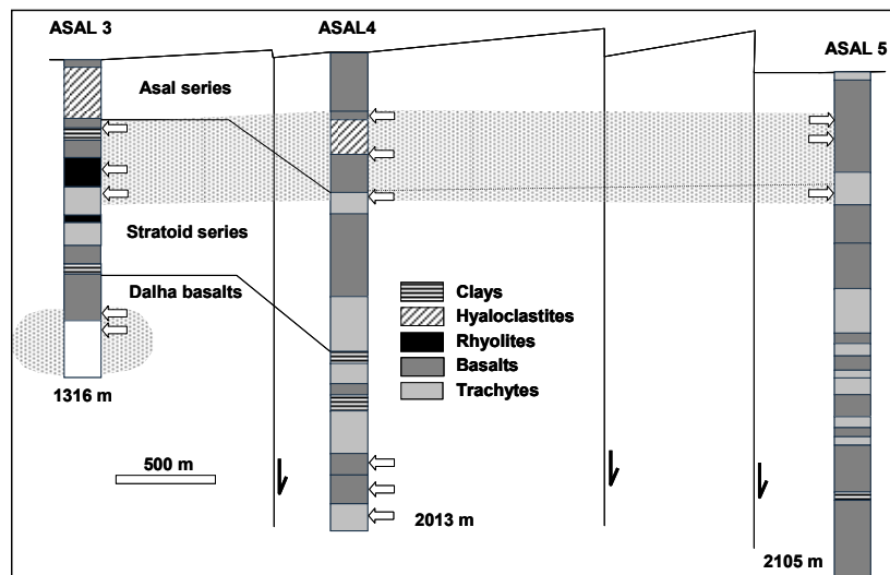
FIGURE 2: Interpreted cross-section in the Asal rift zone
