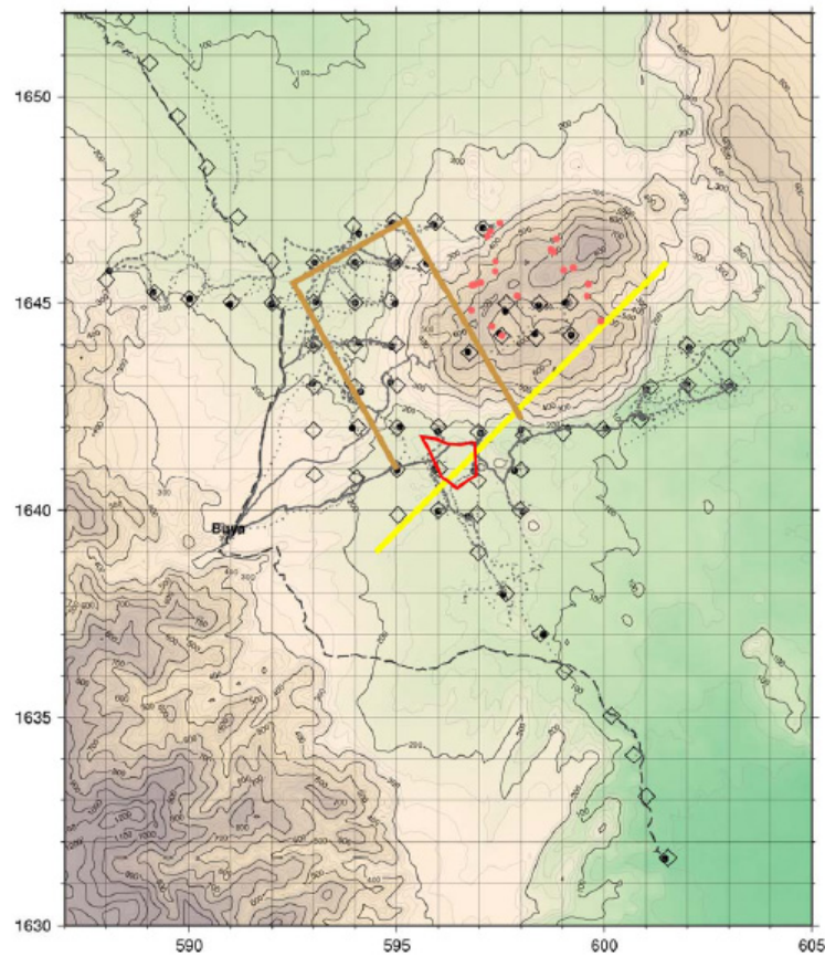
FIGURE 14: The Yellow line shows the location of the vertical resistivity boundary between 1/2 and 2 km depth. The brown contour lines outline the low resistivity body west of Mt. Alid at about 2 km depth. Red dots are geothermal vents on Mt. Alid
