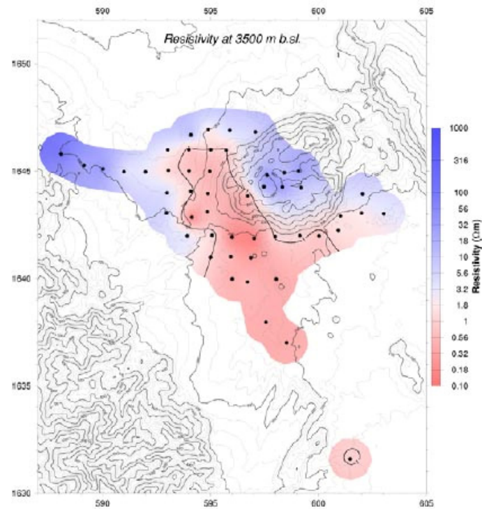
FIGURE 13: Resistivity map at 3500 metres below sea level. Coordinates are in UTM, km units
