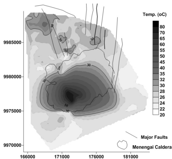
FIGURE 3: Temperature distribution in ^{\circ}\text{C}
