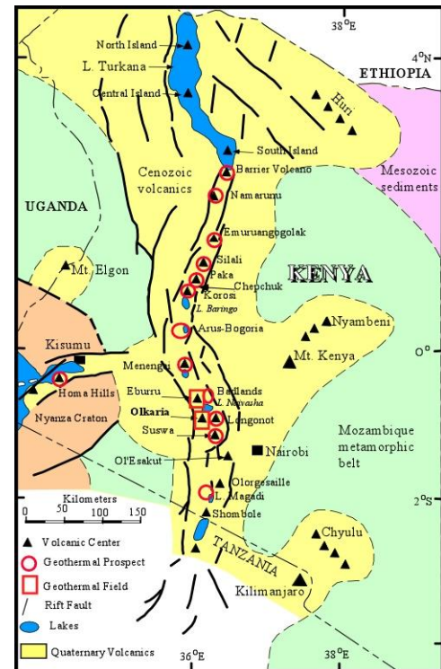
FIGURE 1: Location of Olkaria Geothermal Field within the Kenyan part of the East African Rift
