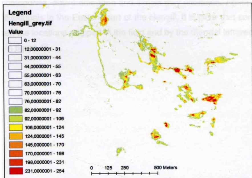
FIGURE 1: Thermal features of the Hengill area. The colours represent represent geothermal activity where the reflective temperature is above 25°C. Red represents the highest temperature. Temperatures lower than 25°C are filtered out
