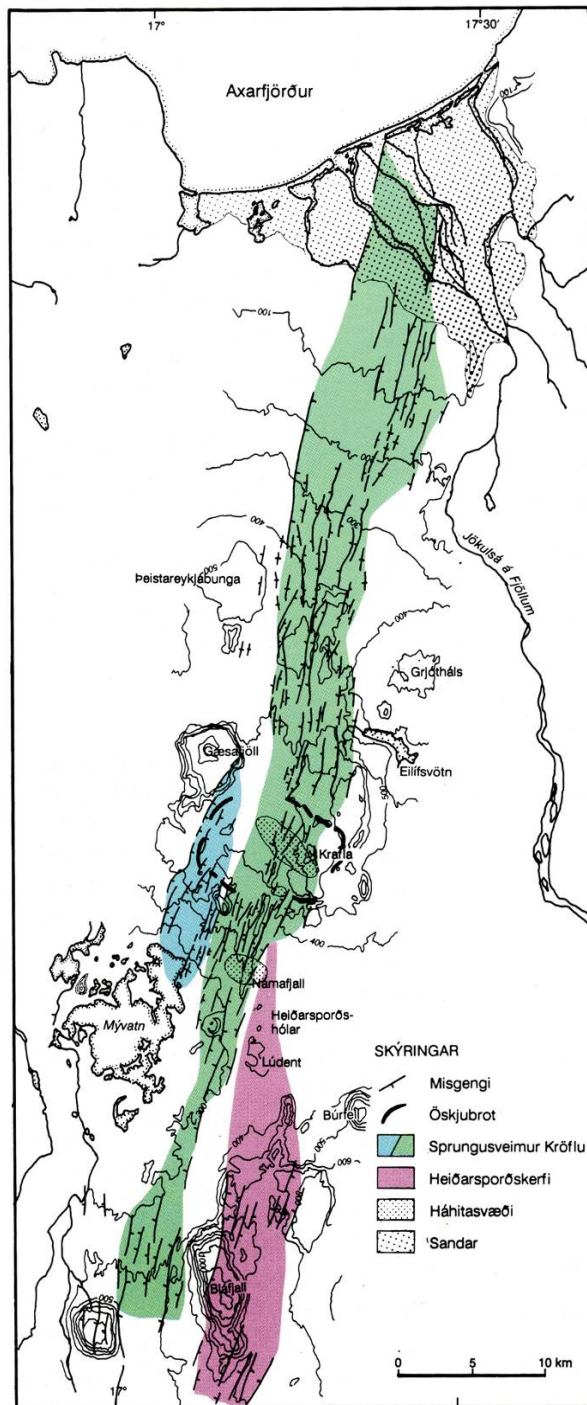
FIGURE 1: Krafla volcanic system. Shield volcano near centre defined by maximum volcanic production (topographical high), silicic rocks a caldera and geothermal activity. It is transected by fissure swarms totalling over 80 km in length, with aligned basaltic crater rows, faults and ground fissures. Volcanic eruptions extend for about 40 km along the swarm. Non-volcanic faults and fissures (surface expression of dykes) extend far beyond surface volcanism
