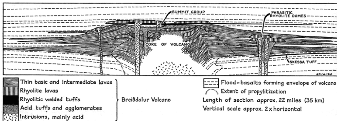
FIGURE 9: Schematic composite section across the Breiddalur central volcano in Iceland, long extinct and exhumed by erosion (Walker 1963). A caldera in the core area of the volcano once hosted a geothermal system of which high-temperature alteration is evidence. Intrusive complex is found in roots of volcano
