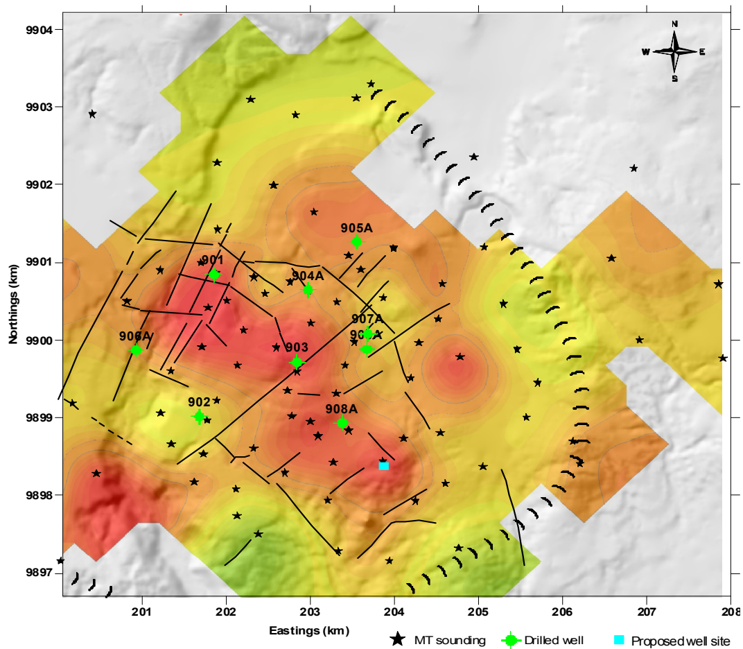
FIGURE 1: MT resistivity iso anomaly map at 700 masl (meters above sea level) of Domes area.
