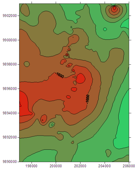
FIGURE 2: Gravity contour map of Longonot, Suswa and Olkaria showing the variation of the gravity anomalies in the area
