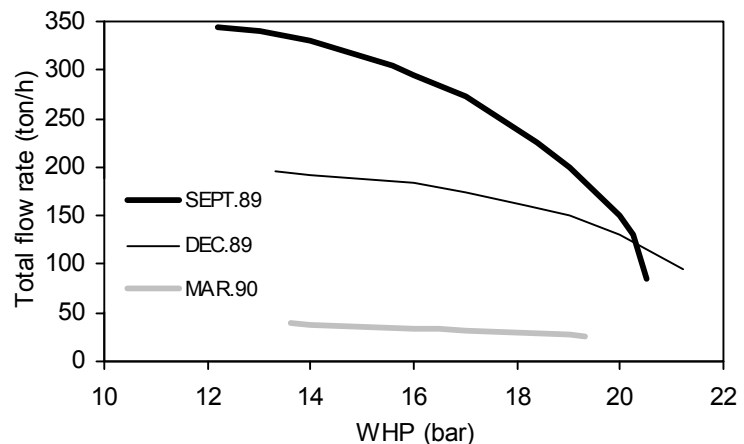
FIGURE 3: Successive output curves of the well Asal 3
