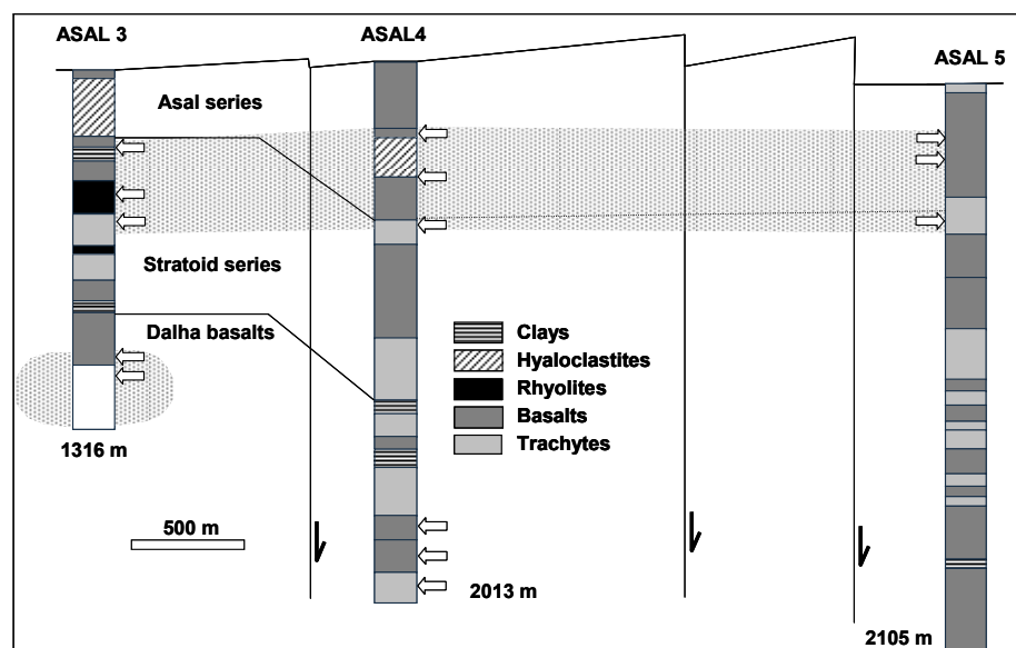
FIGURE 2: Interpreted cross-section from the Asal rift zone
