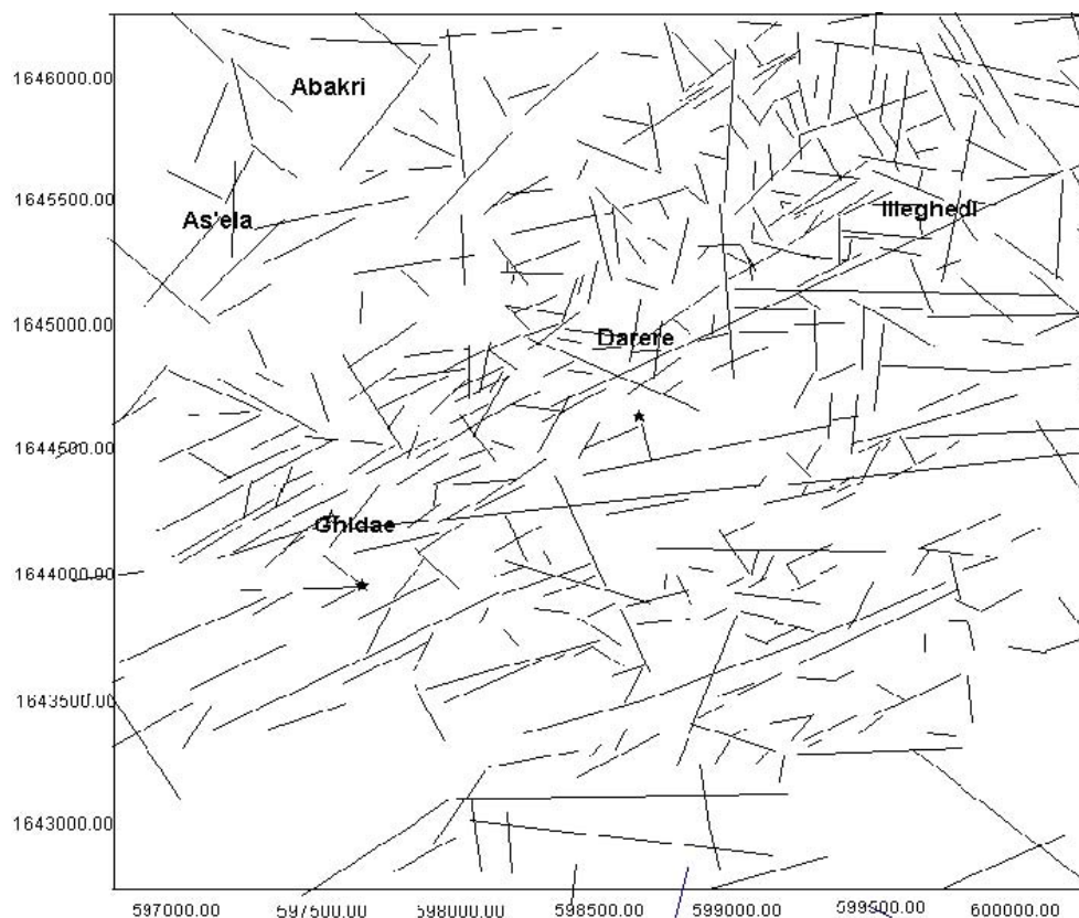
FIGURE 9: Lineaments interpreted mainly from 1:20000 aerial-photograph and digital images
