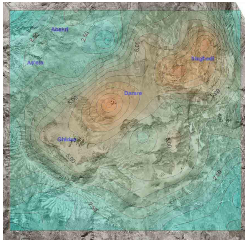
FIGURE 10: Contour plot of Alid area using FFD analysis. Note the high values lie on the Darara-Illeggedi line. It is superimposed on aerial photo.
