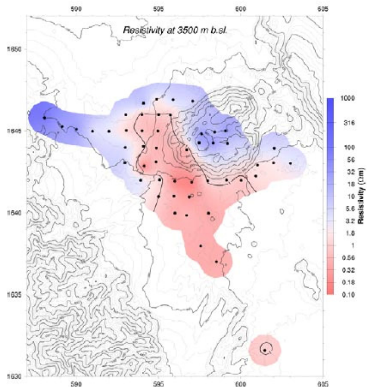
FIGURE 12: Resistivity map at 3500 metres below sea level. Coordinates are in UTM, km units
