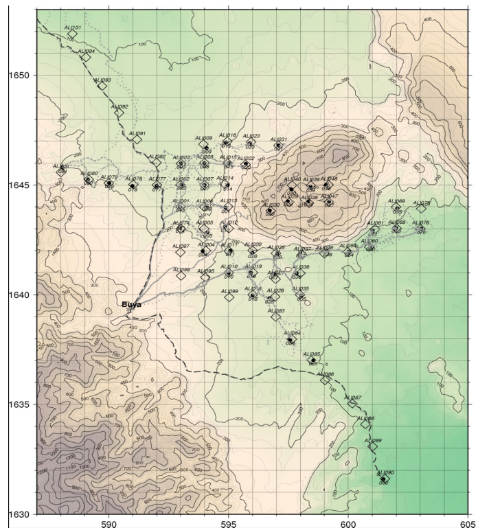
FIGURE 11: Location of TEM (open diamond) and MT soundings (filled circles). Coordinates are in UTM, km units.
