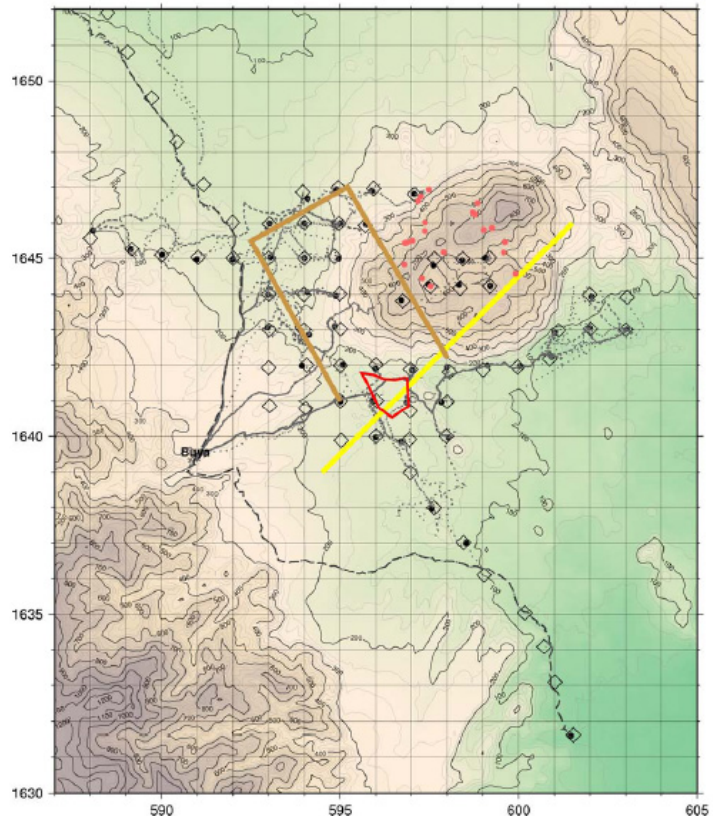
FIGURE 13: The yellow line shows the location of the vertical resistivity boundary between ½ and 2 km depth. The brown contour lines outline the low resistivity body west of Mt. Alid at about 2 km depth. Red dots are geothermal vents on Mt. Alid
