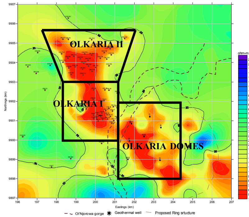
FIGURE 3: Map showing TEM Resistivity at 1000 m a.s.l.
