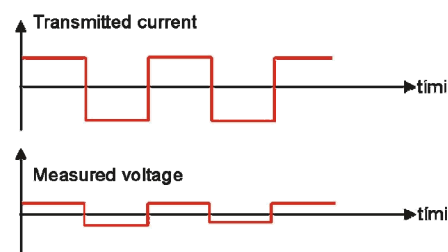
FIGURE 2: The principles behind the Schlumberger configuration and the associated current distribution in the earth
