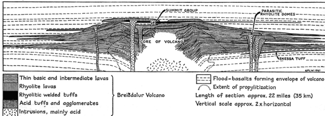
FIGURE 9: Schematic composite section across the Breiddalur central volcano in Iceland, long extinct and exhumed by erosion (Walker 1963). A caldera in the core area of the volcano once hosted a geothermal system of which high-temperature alteration is evidence. Intrusive complex is found in roots of volcano
