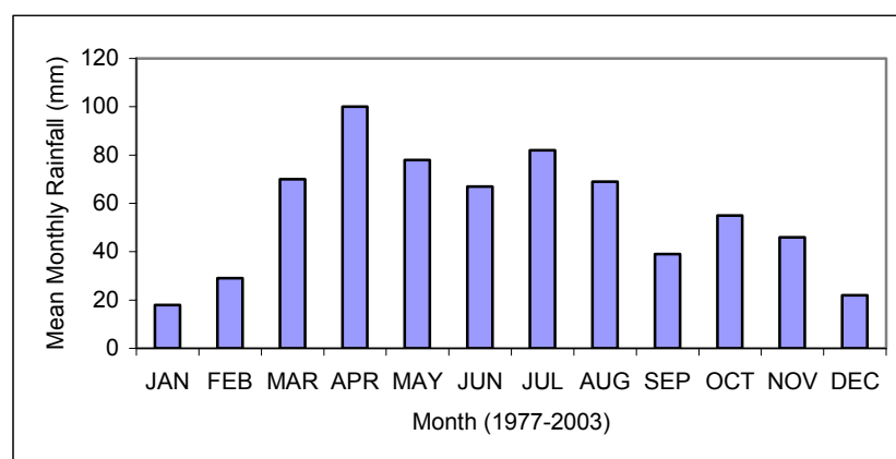
FIGURE 1: Lake Bogoria mean monthly Rainfall at Loboï Station from 1977-2003
