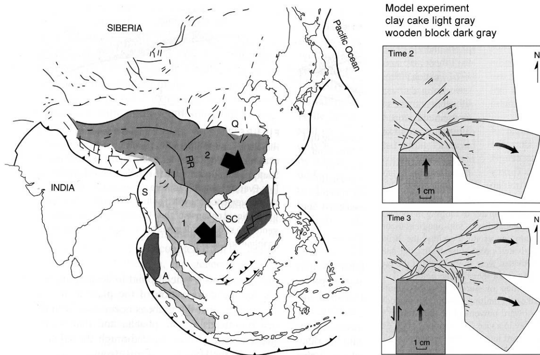
FIGURE 5: Tectonics of SE-Asia showing eastward escape of large crustal blocks along major strike-slip faults as suggested by Tapponier et al. (1982). Model for comparison (from Pluijm and Marshak, 2004)
