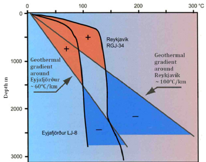
FIGURE 3: Reykjavík and Akureyri, Iceland. Bold lines show actual reservoir temperature, 130-140°C for Reykjavík, 90-95°C for Akureyri. Water transports heat from deep levels, thus cooling the rock (heat mining). Shallower levels consequently are heated up
