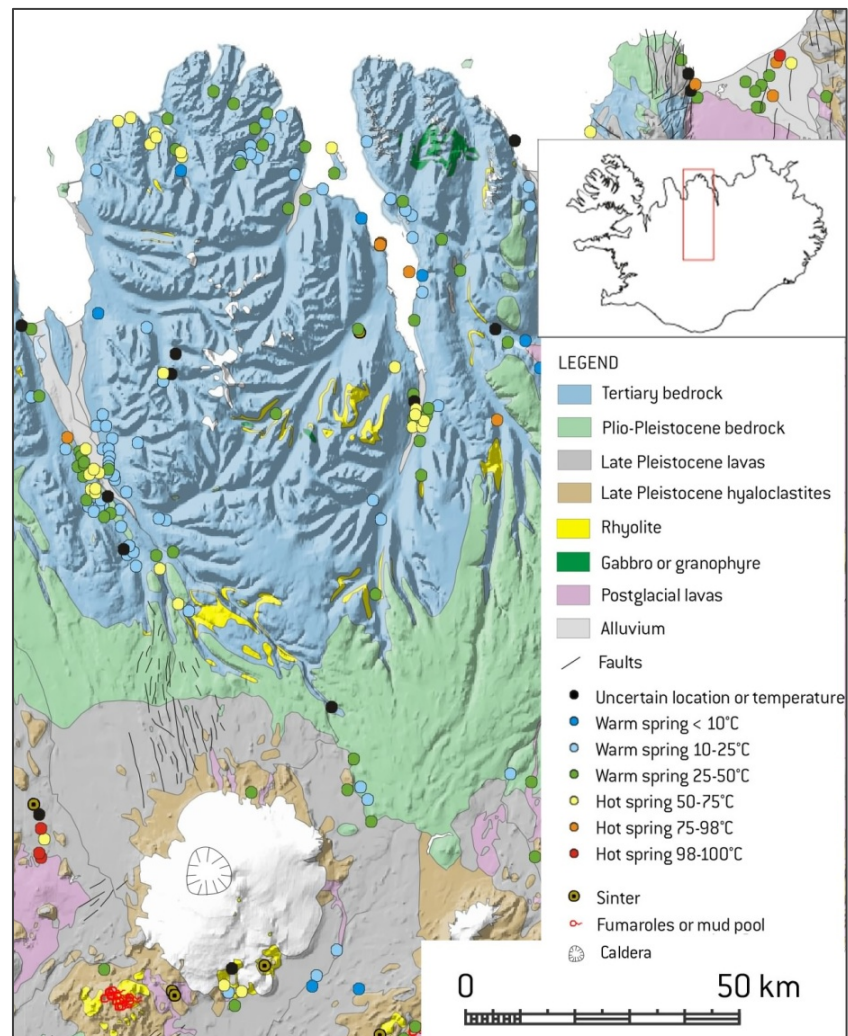
FIGURE 4: Hofsjökull volcano in central Iceland. A fissureswarm extends about 90 km to the NNW from it. Fissure eruptions occur along the first 30 km (proximal part). Faults and fissures extend another 60 km beyond with numerous hot springs in valleys eroded into 7-8Ma basalts (distal part)
