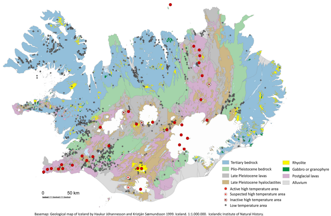
FIGURE 1: Geothermal map of Iceland. High-temperature fields inside the active volcanic zone are shown as red circles, and hot and warm springs as dark circles
