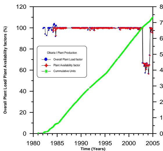
FIGURE 15: Olkaria I Plant Production
