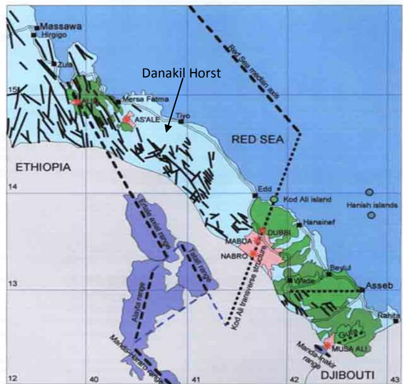
Figure 4. Structural features of the southwestern Red Sea coastal region and the distribution of Tertiary and Quaternary volcanic rocks in southeast Eritrea
