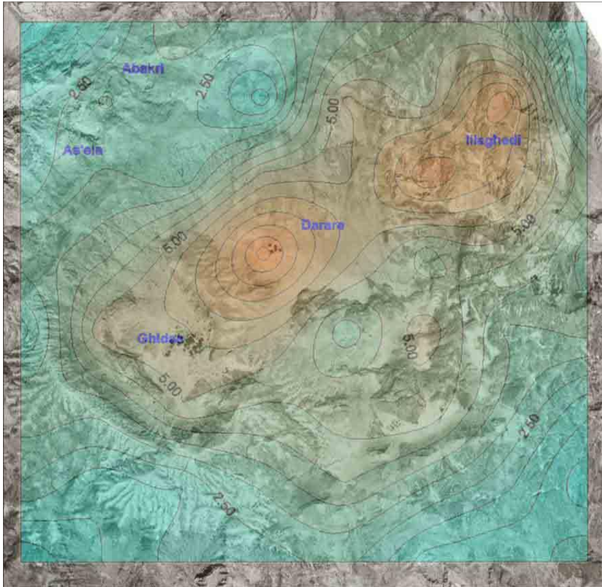
FIGURE 10: Contour plot of Alid area using FFD analysis. Note the high values lie on the Darere-Illegbedi line. It is superimposed on aerial photo
