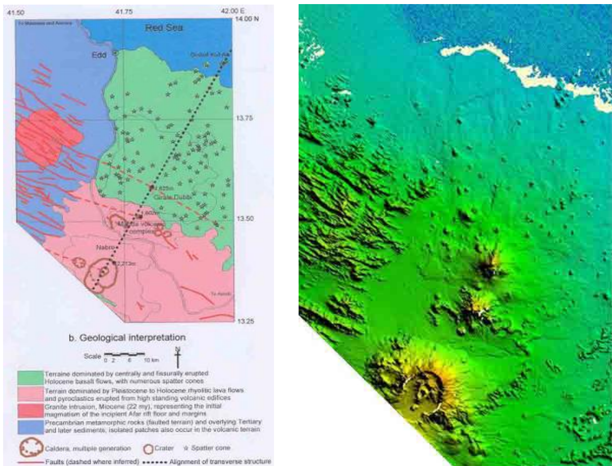
FIGURE 6: Geological interpretation of Nabro-Dubbi area, notice the intersection of structures. The right photo is the the DEM of the Nabro-Dubbi (DOM, 2004)
