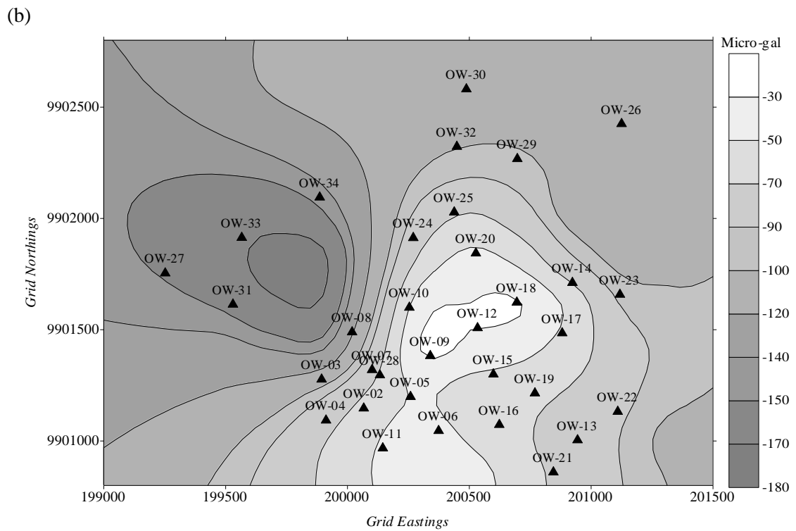
FIGURE 4: Gravity changes over Olkaria 1 geothermal field between 1983 and 1988 (a), and between 1988 and 2000 (b)
