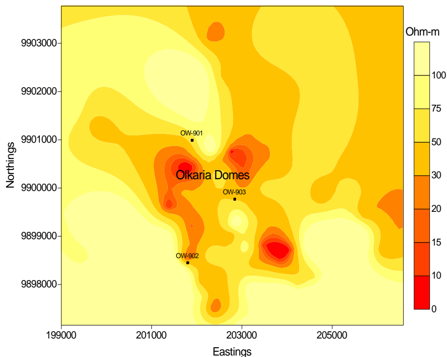
FIGURE 7: MT Resistivity distribution at 1000 mbsl around Olkaria-Domes geothermal field and its surroundings
