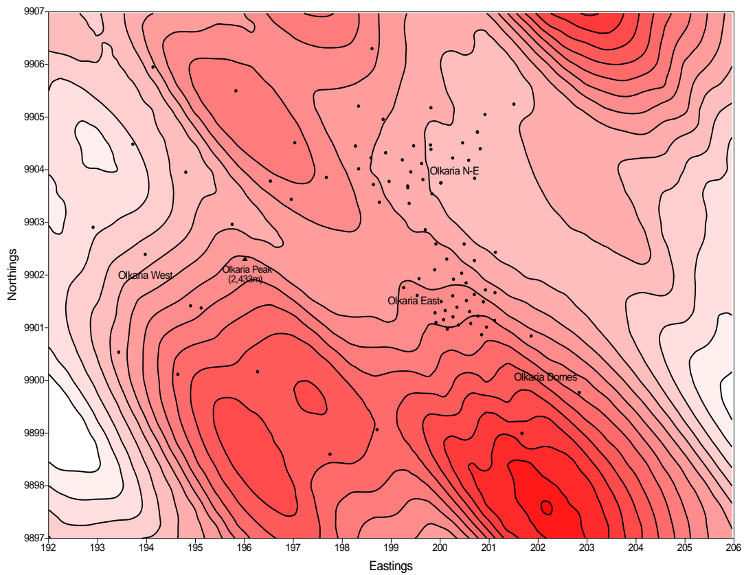
FIGURE 3: Directionally filtered gravity data of the greater Olkaria geothermal field. This procedure highlights the NW-SE trend of the gravity anomaly through Olkaria, not seen in the Bouguer data in Figure 2
