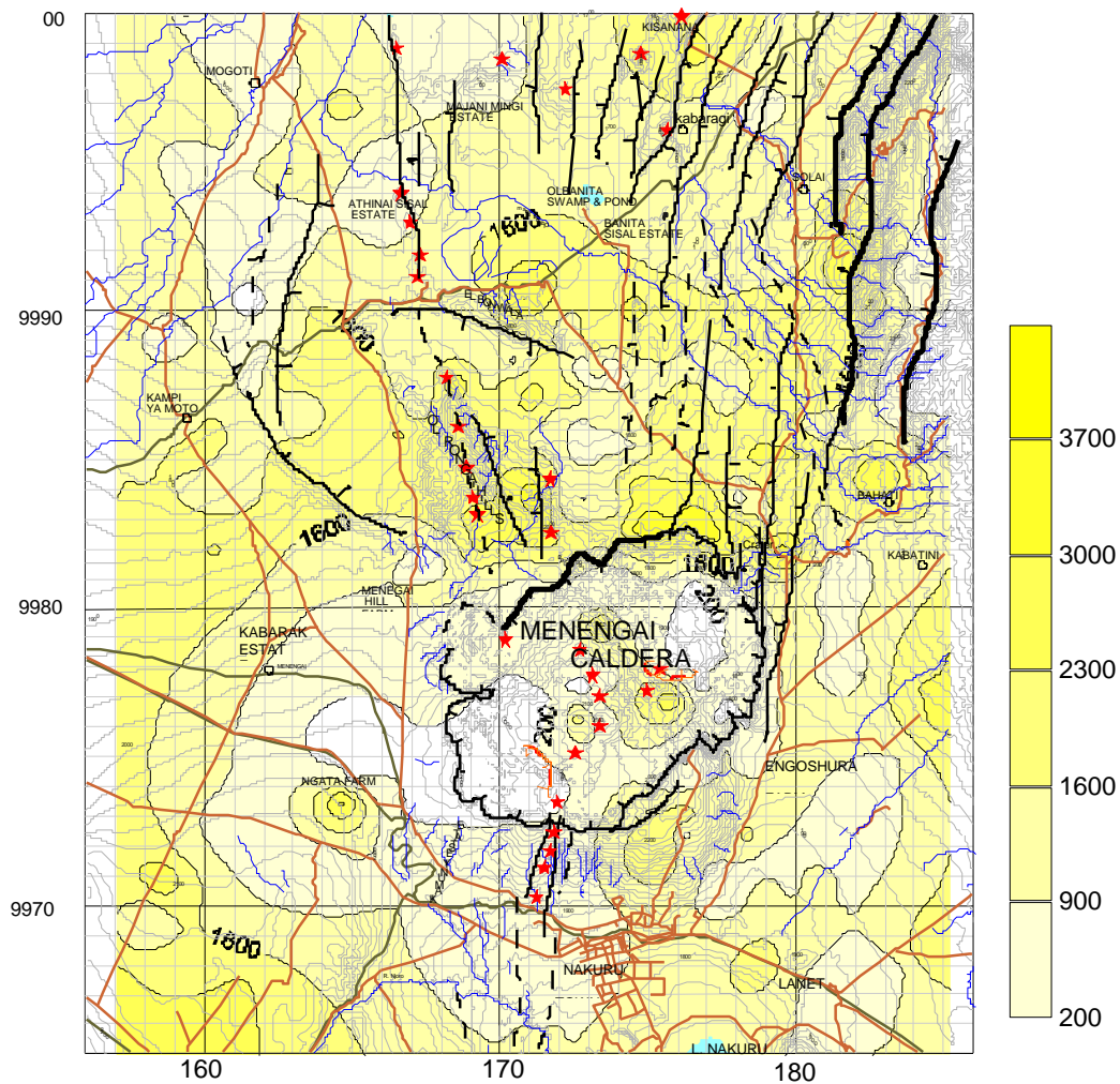
FIGURE 4: Radon radioactivity distribution in the Menengai prospect area
