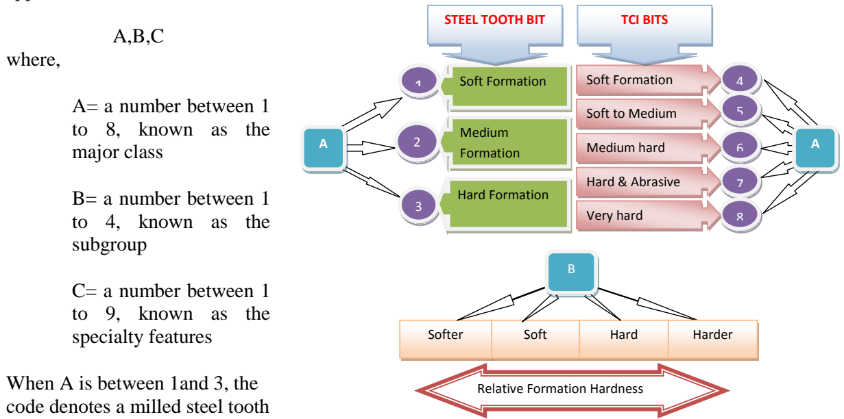
FIGURE 10: Bit Classification
