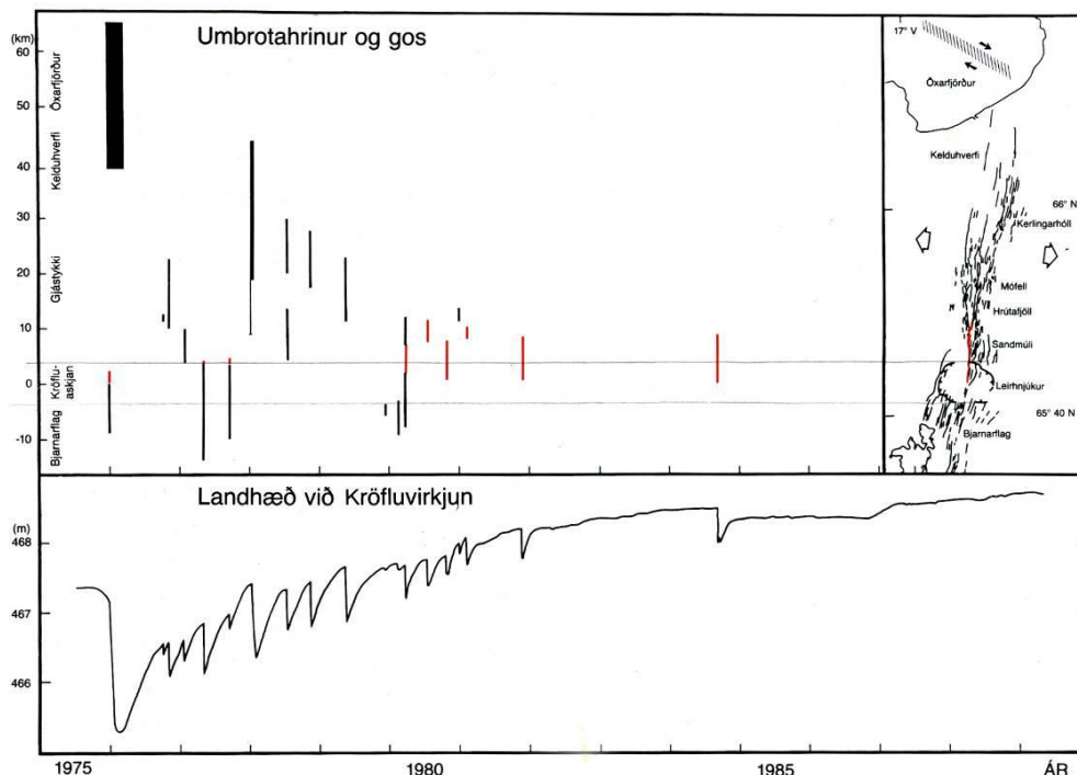
FIGURE 9: Krafla rifting episode of 1975-1984. Course of events. Upper diagram: Dyking (black) and eruptive events (red). The bars indicate the part of the fissure swarm which were affected in individual events with reference to the map on the right. Their thickness is proportional to the time each event lasted. Lower diagram: elevation changes with time (Einarsson 1991)
