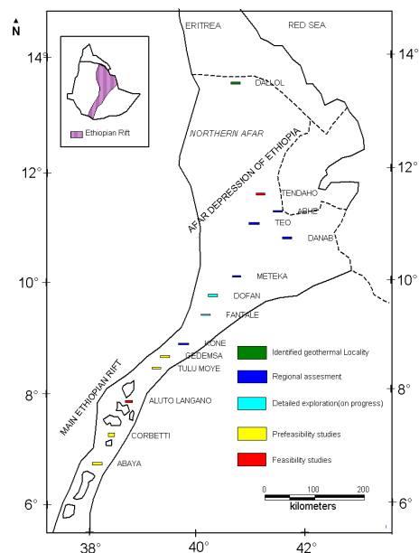
FIGURE 6: Location map of the geothermal areas in the Ethiopian Rift
