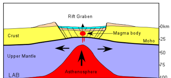
FIGURE 2: Generalized E-W section across a typical continental rift showing late stages of its formation
