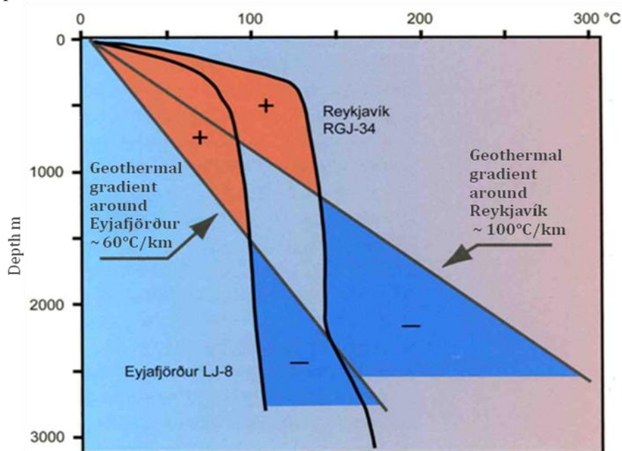
FIGURE 1: Reykjavík and Akureyri, Iceland. Bold lines show actual reservoir temperature, 130-140°C for Reykjavík, 90-95°C for Akureyri. Water transports heat from deep levels, thus cooling the rock (heat mining). Shallower levels consequently are heated up
