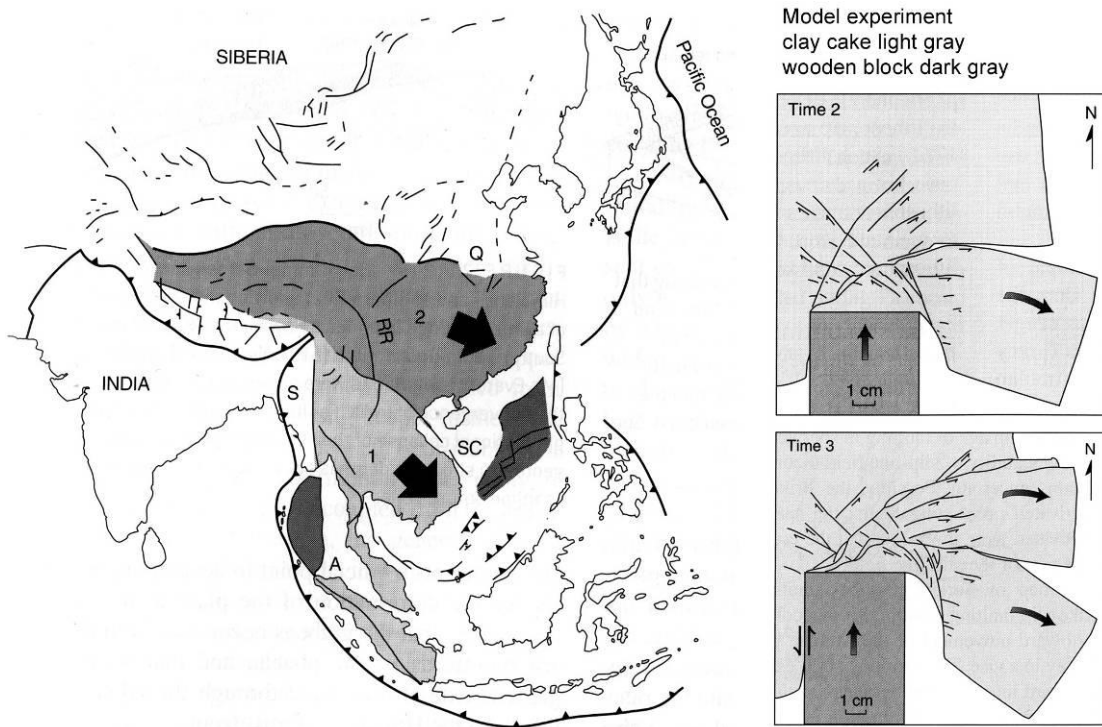
FIGURE 3: Tectonics of SE-Asia showing eastward escape of large crustal blocks along major strike-skip faults as suggested by Tapponier et al. (1982). Model for comparison (from Pluijm and Marshak 2004)
