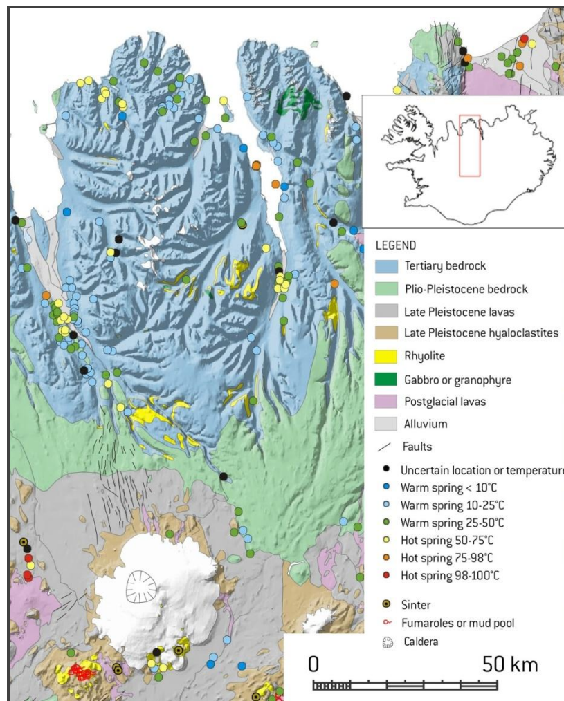
FIGURE 2: Hofsjökull volcano in central Iceland. A fissure swarm extends about 90 km to the NNW from it. Fissure eruptions occur along the first 30 km (proximal part). Faults and fissures extend another 60 km beyond with numerous hot springs in valleys eroded into 7-8Ma basalts (distal part)
