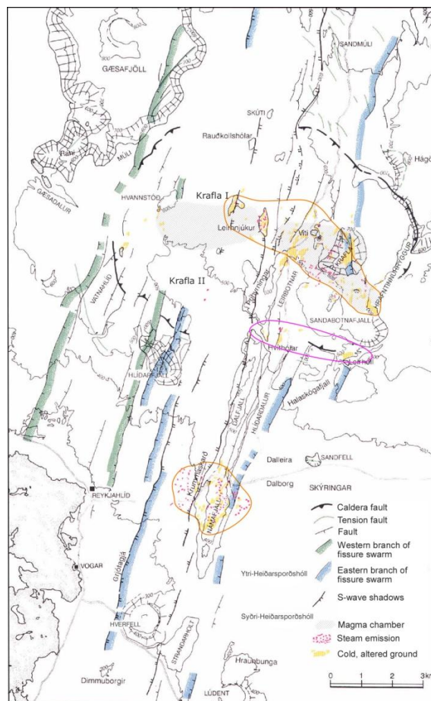
FIGURE 5: Central part of Krafla volcanic system showing caldera and fissure swarms which traverse it. The Krafla caldera hosts a geothermal system. It has a magma chamber (S-wave shadow) at 3-7 km depth. A second geothermal area at Námafjall on the fissure swarm 7 km south of Krafla is located where basaltic fissure eruptions concentrate
