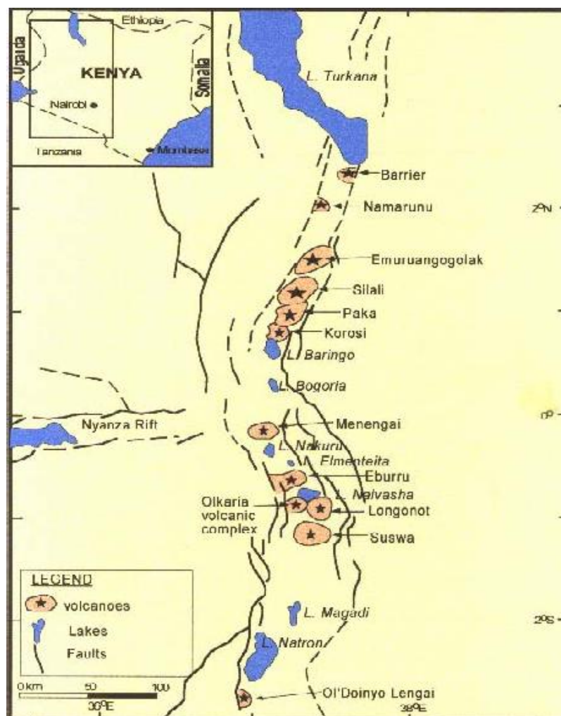
FIGURE 6: Apex of Kenya Rift domal uplift with two volcanically active rift branches and a third E-W branch dying. Stratovolcanoes are shown. Fissure swarms have not been identified as integral parts of volcanic systems (Mwawongo 2004)
