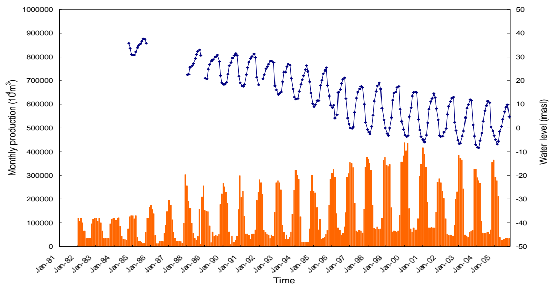
FIGURE 1: Water level monitoring data in Xiaotangshan geothermal field
