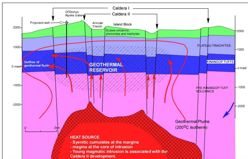
FIGURE 13: Geothermal model of Suswa volcano
