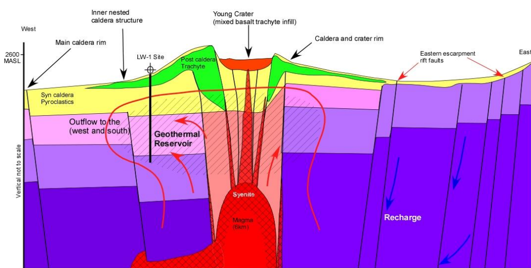
FIGURE 10: Geothermal model of Longonot Volcano
