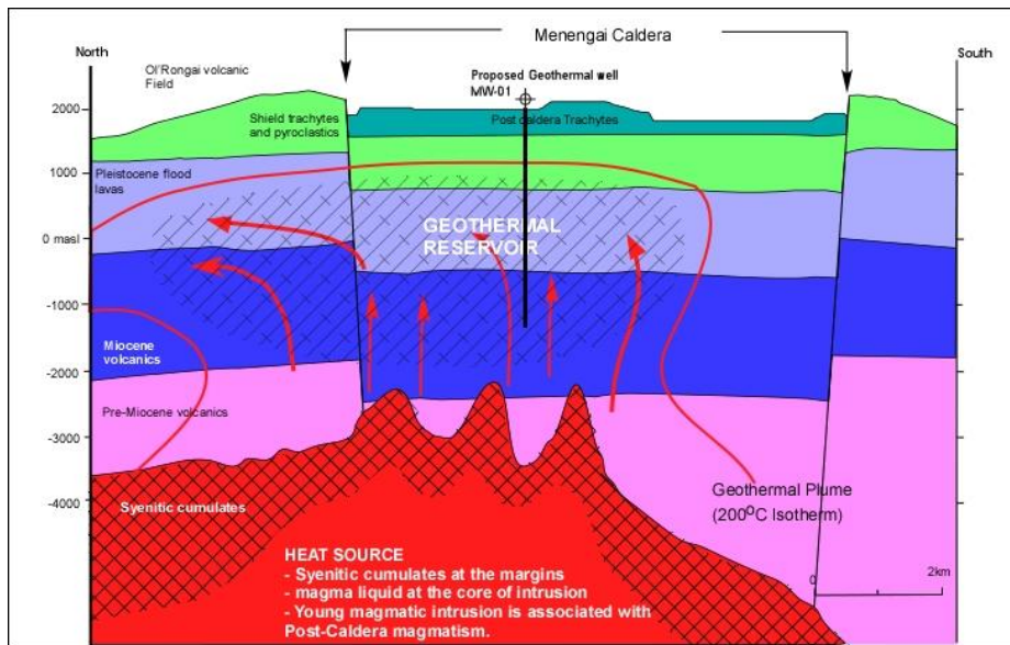
FIGURE 7: Geothermal model of Menengai volcano
