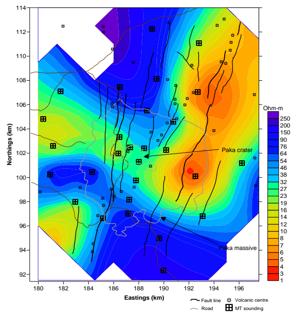
FIGURE 21: MT resistivity plot at 3000mbsl
