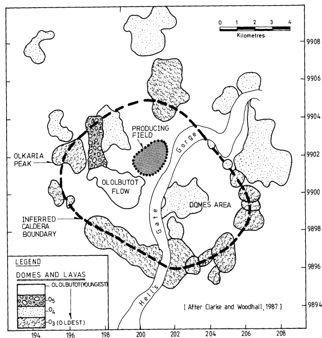
FIGURE 6: Map showing Ololbutot lava flow in relation to the production field (Olkaria I)
