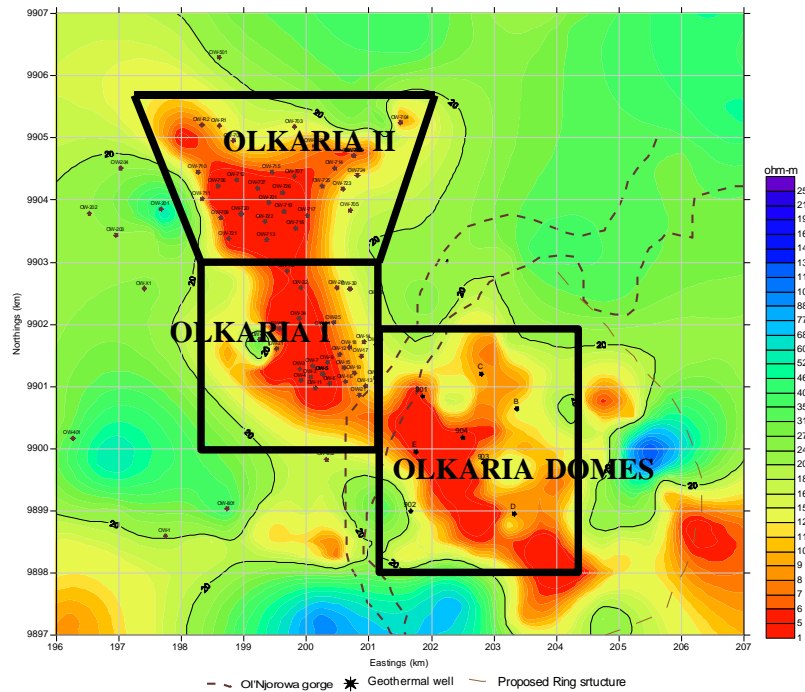
FIGURE 5: Map showing TEM Resistivity at 1000 m a.s.l.
