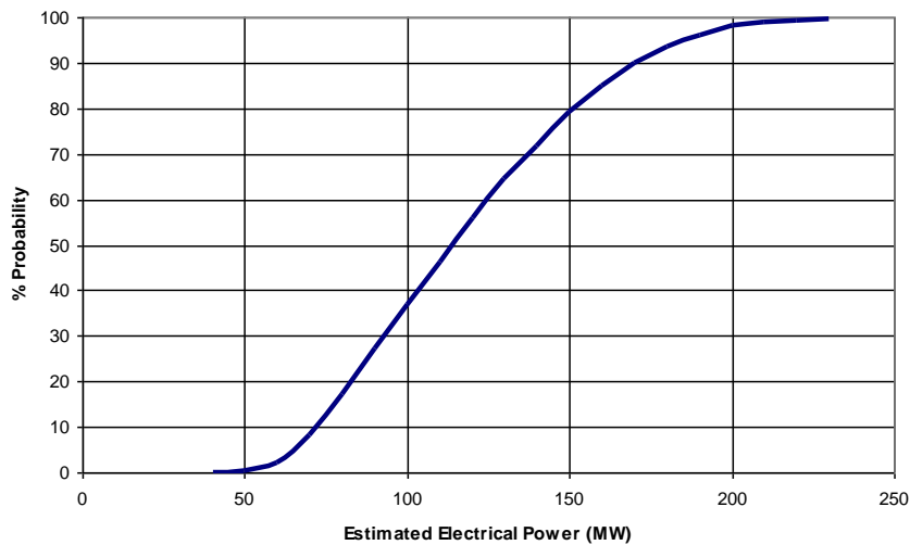
FIGURE 7: Frequency distribution of Power Capacity
