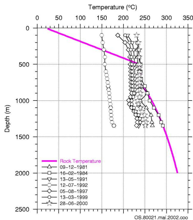
FIGURE 2: Temperatures in well OW-21, a typical Olkaria I profile
