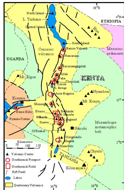
FIGURE 1: Location of Olkaria Geothermal Field within the Kenyan part of the East African Rift
