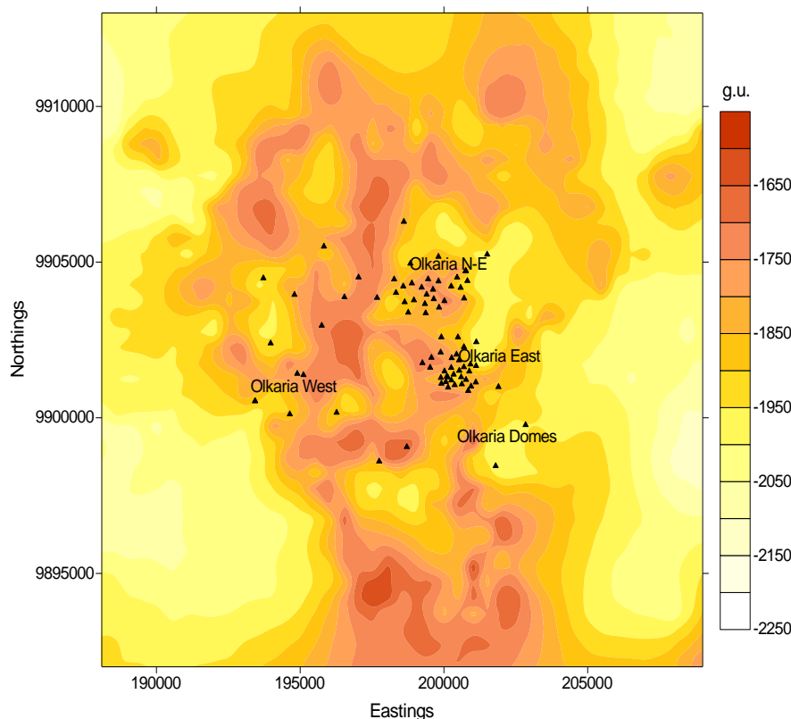
FIGURE 6: Gravity distribution at the Olkaria area
