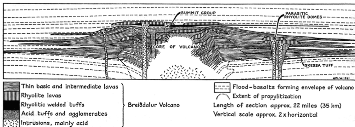
FIGURE 8: Schematic composite section across the Breiddalur central volcano in Iceland, long extinct and exhumed by erosion (Walker 1963). A caldera in the core area of the volcano once hosted a geothermal system of which high-temperature alteration is evidence. Intrusive complex is found in roots of volcano.
