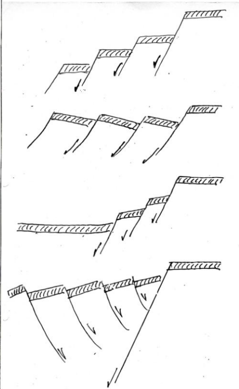
FIGURE 3: Types of faults
