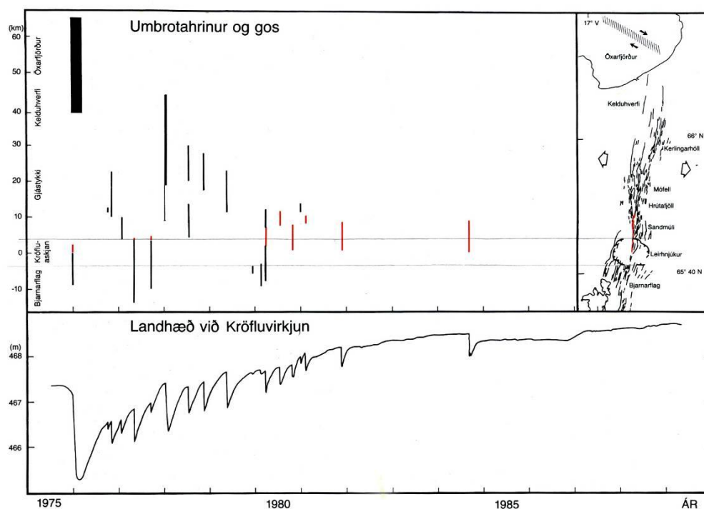
FIGURE 9: Krafla rifting episode of 1975-1984. Course of events. Upper diagram: Dyking (black) and eruptive events (red). The bars indicate the part of the fissure swarm which were affected in individual events with reference to the map on the right. Their thickness is proportional to the time each event lasted. Lower diagram: elevation changes with time (Einarsson 1991).
