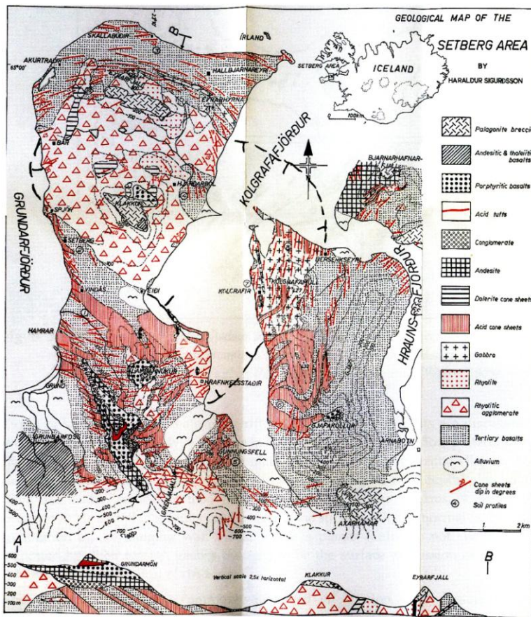
FIGURE 2: Cone sheet swarm of Setberg volcanic centre, West Iceland. The sheets are inclined 25-40° towards a focus at about 3 km depth underneath a caldera filled with silicic breccia and a gabbro intrusion (Sigurdsson 1967).
