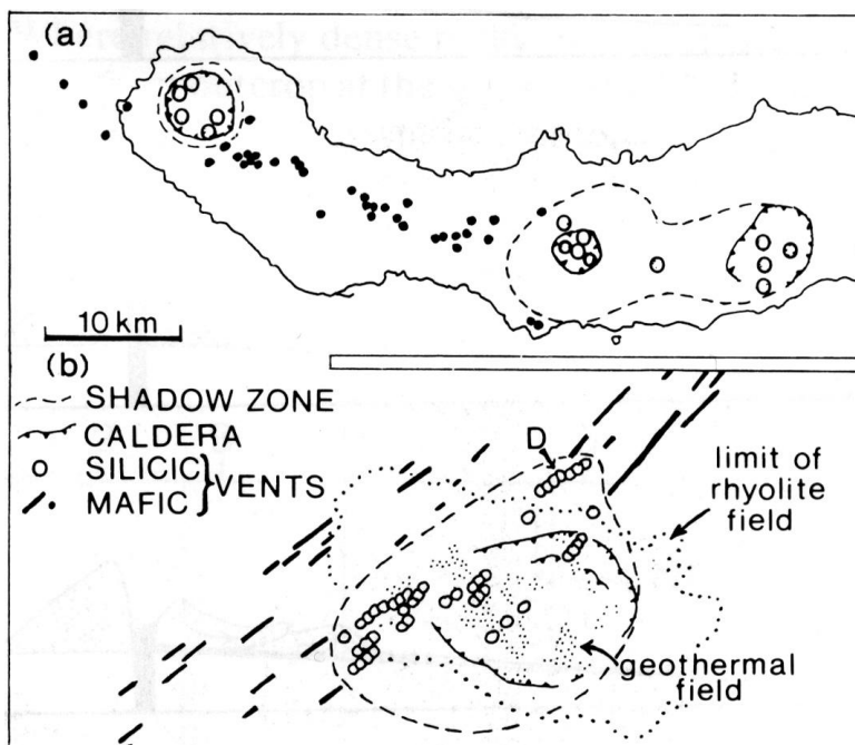
FIGURE 4: Examples of magmatic shadow zones (where basalt does not erupt) in calderas of rhyolite volcanoes. Magma chambers with silicic melts prevent basaltic magmas from attaining the surface. Such erupt on the adjoining fissure swarms (Walker 1989).
