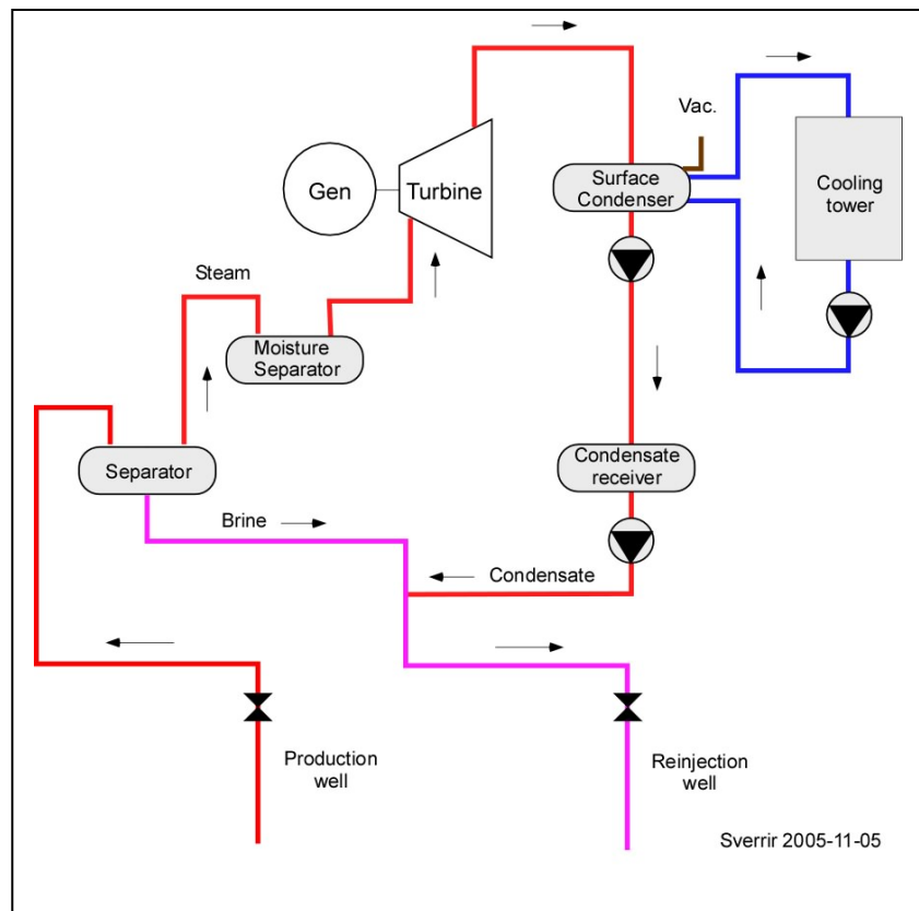
FIGURE 2: Sketch of the fluid path of a conventional geothermal
