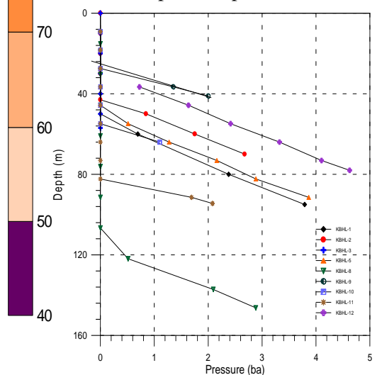
FIGURE 11: Downhole pressure profiles
