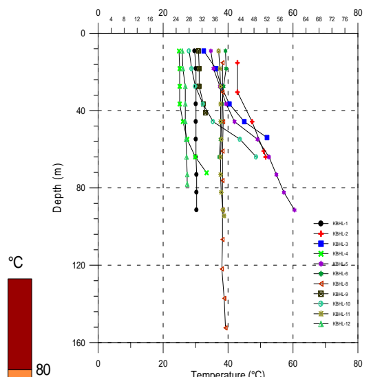
FIGURE 10: Downhole temperature profiles
