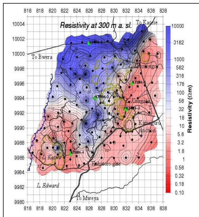
FIGURE 3: Katwe, resistivity at 300 m a.s.l. (from Gíslason et al., 2005)
