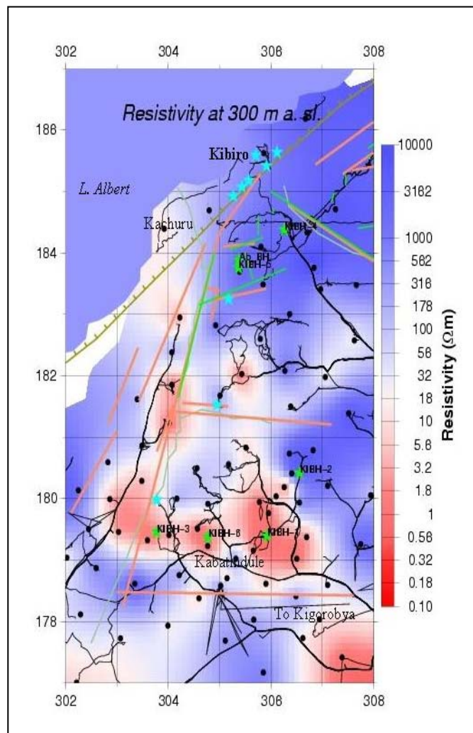
FIGURE 6: Kibiro, resistivity at 300 m a.s.l., faults and fractures, geothermal surface manifestations (stars) (from Gíslason et al., 2005)
