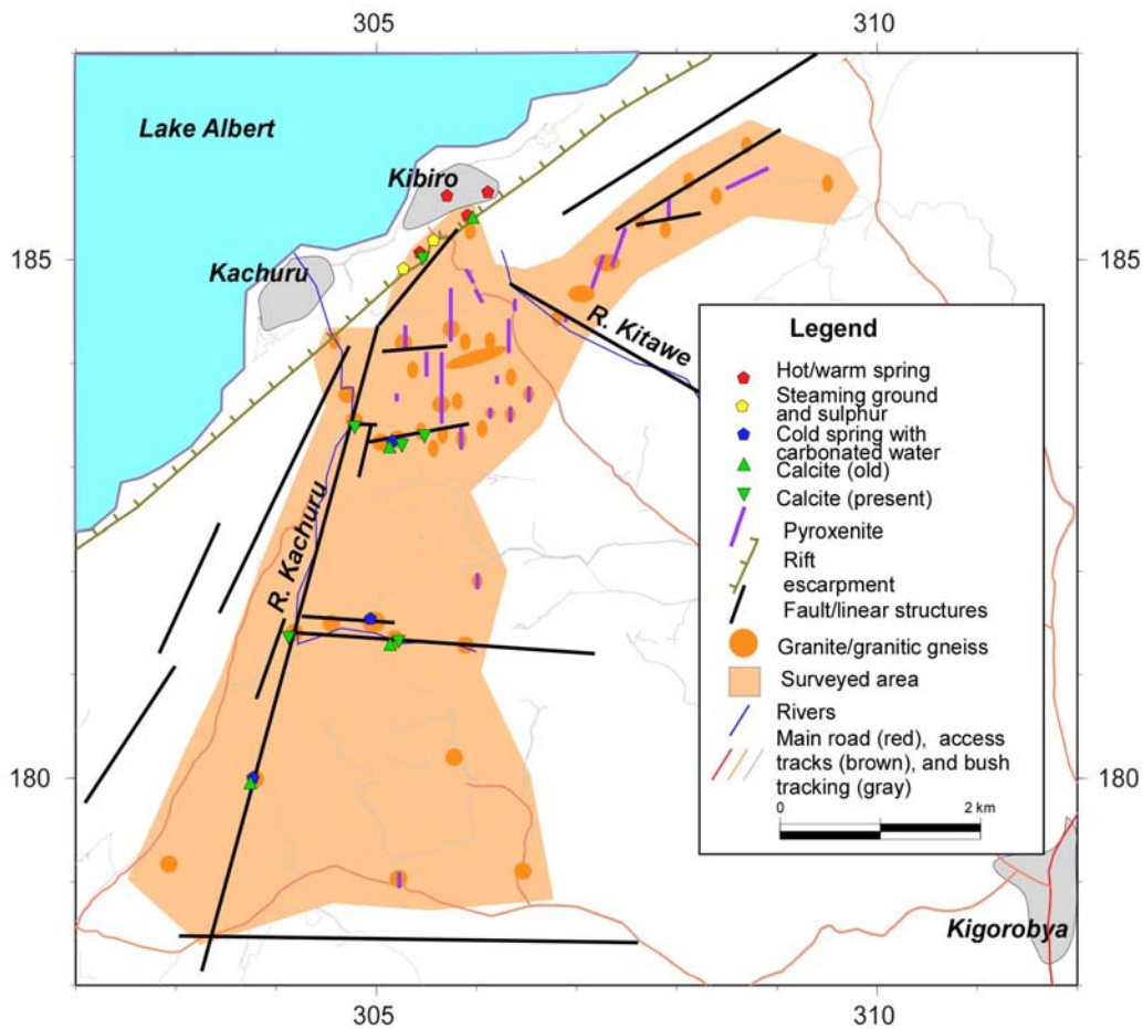
FIGURE 4: Kibiro, geology and geothermal surface manifestations (from Gíslason, et al., 2004)
