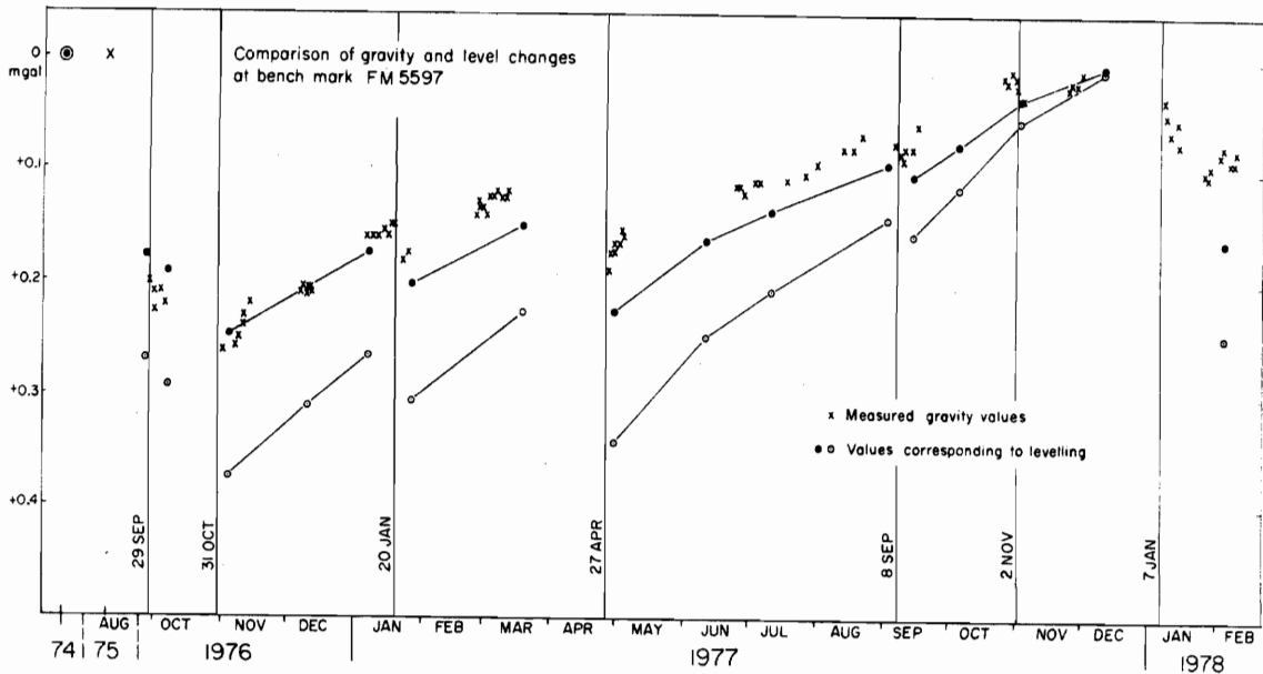
Fig. 8: Comparison of gravity and level changes with time at benchmark FM-5597. For location see Fig. 5. Crosses show measured gravity values. Filled circles show gravity calculated from measured level values assuming the Bouguer model ( 0.01 \text{ mgal} \approx 3 \text{ cm} ). Open circles show gravity values corresponding to measured level values using the free air model ( 0.01 \text{ mgal} \approx 5 \text{ cm} ).
